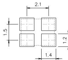
Reference Footprint
